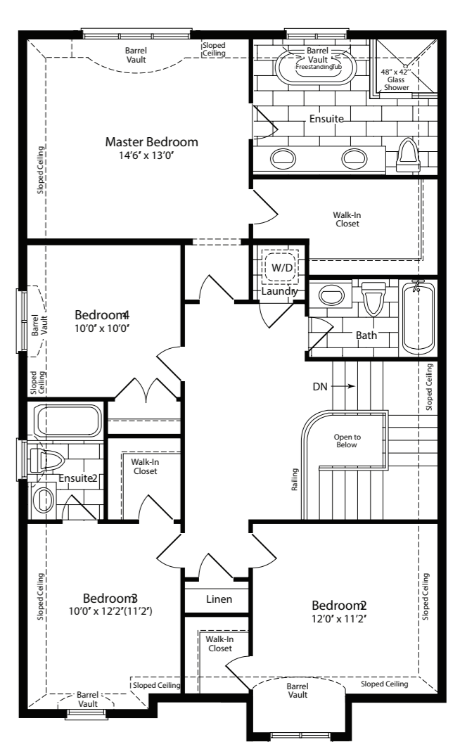
Third Floor Plan Elev. B
