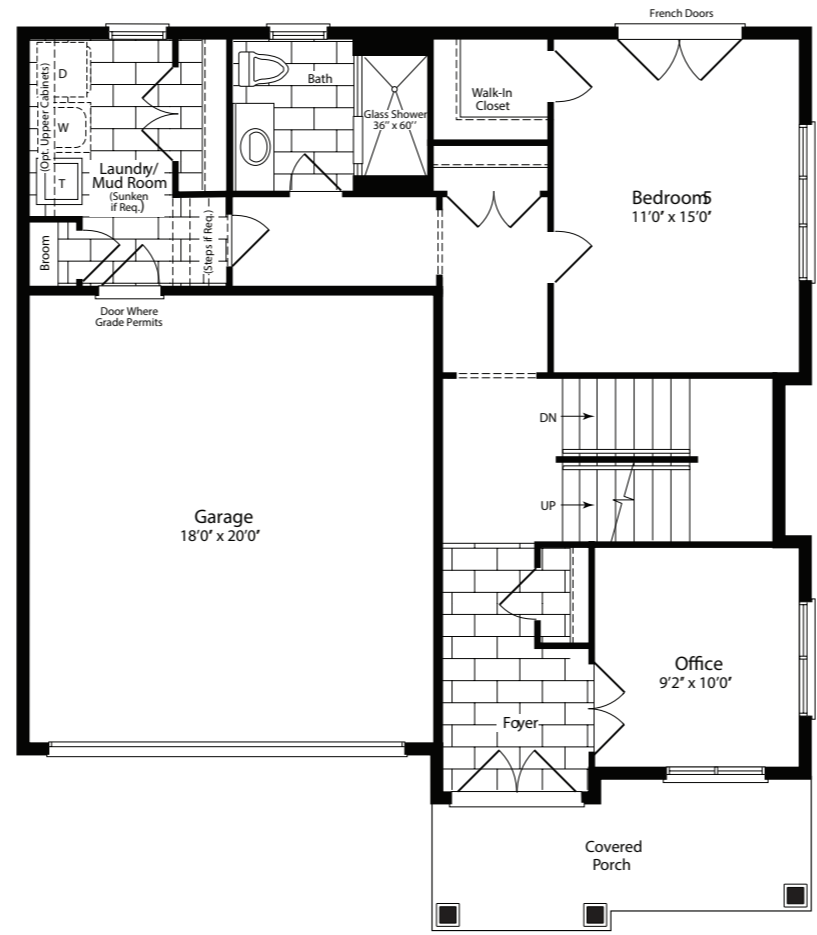
Ground Floor Plan Elev. A
