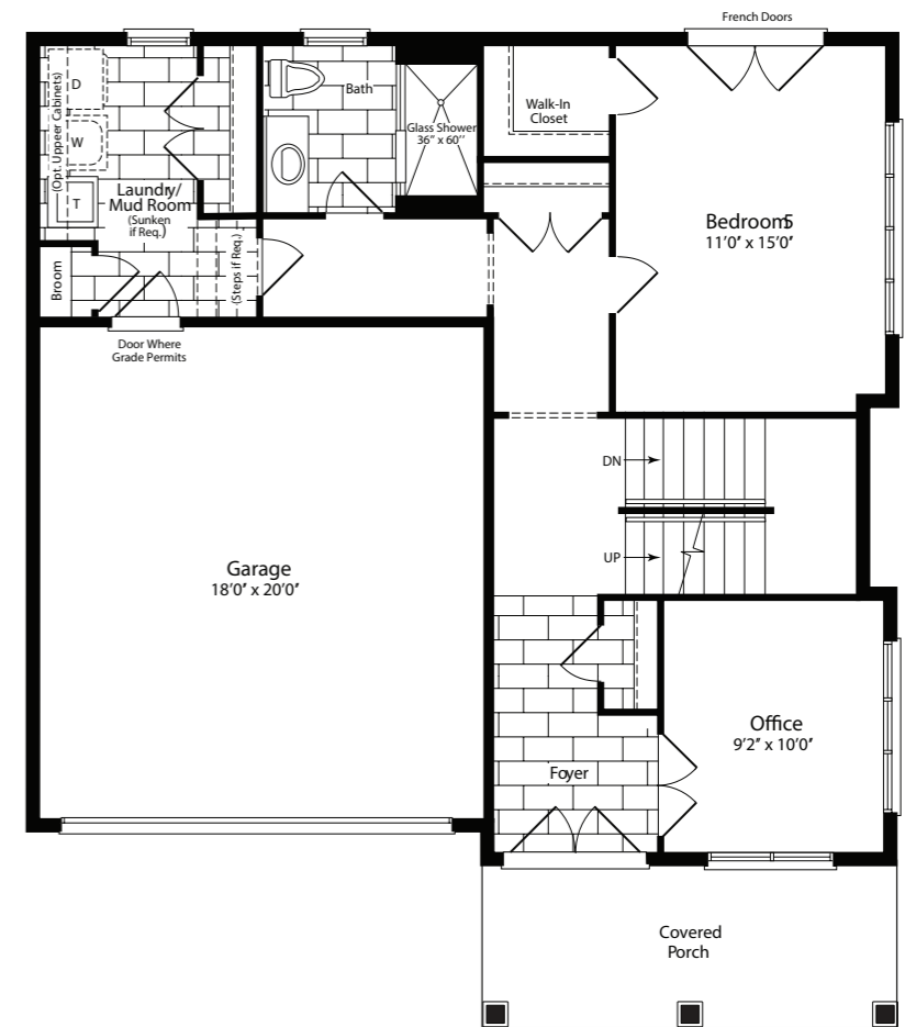
Ground Floor Plan Elev. B
