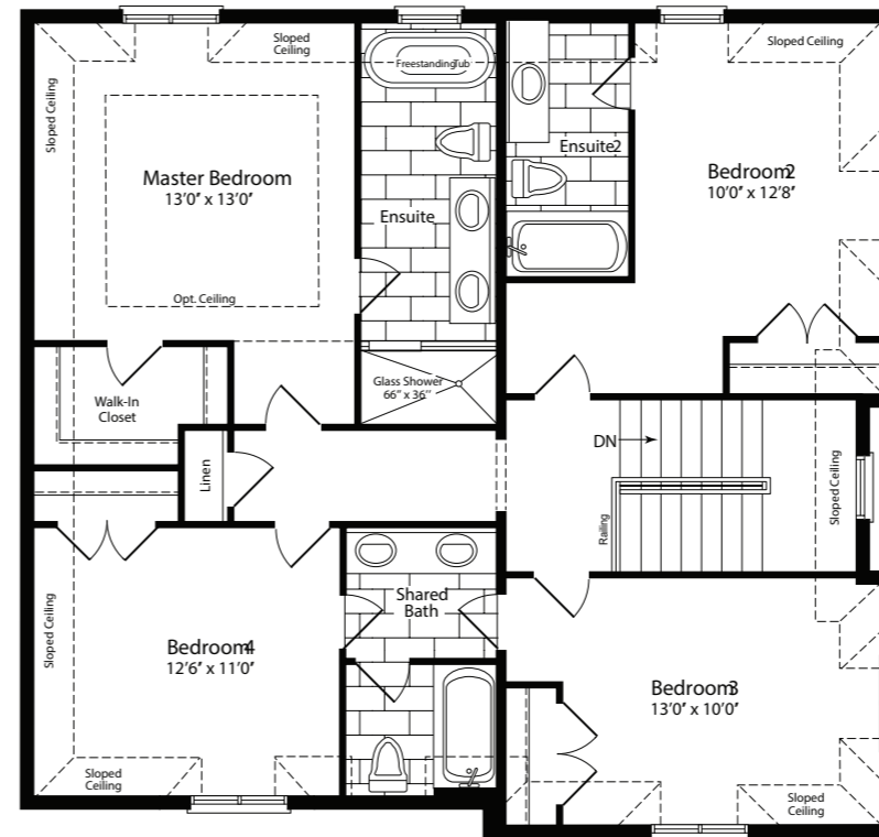
Third Floor Plan Elev. A
